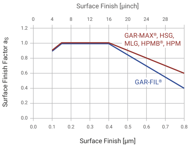
Fig. 12: Mating Surface Factor a_S
