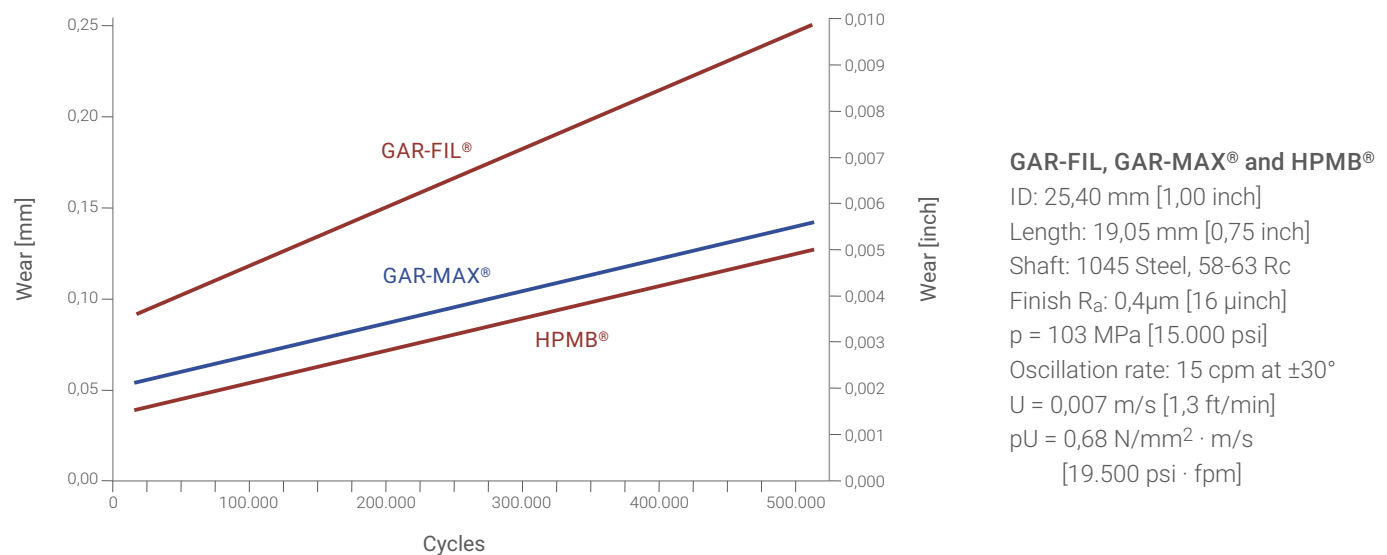
Fig. 3: Wear rate for GAR-FIL, GAR-MAX and HPMB
