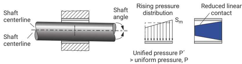
Fig. 16: Slight misalignment
